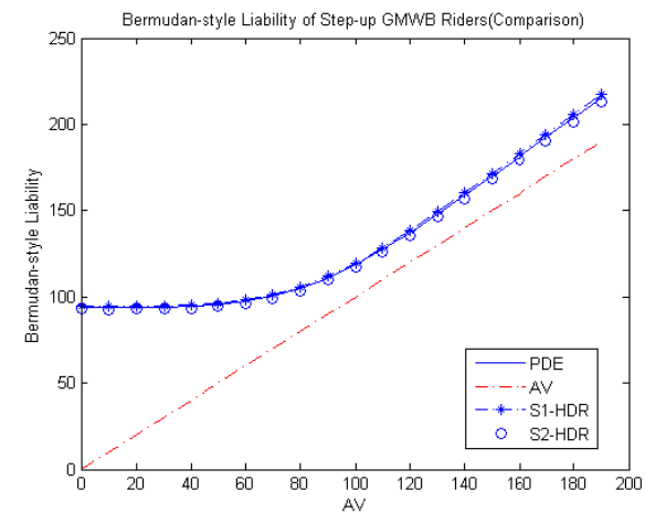
Fig. 4. Consistency of PDE scheme and HDR scheme (S1 and S2) when r(0) = 2\%
