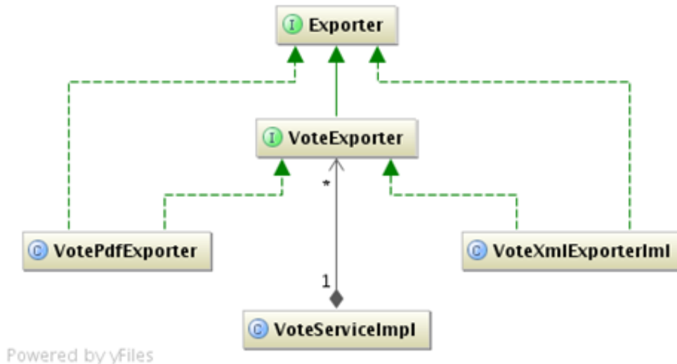
Fig. 8. Repository of the Vote Exporters in UML
