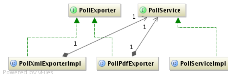
Fig. 7. Typical dependencies between classes from the Service project in UML
