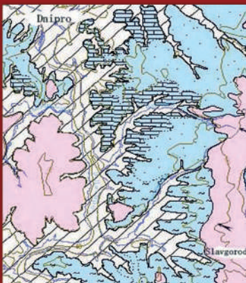
Geology
