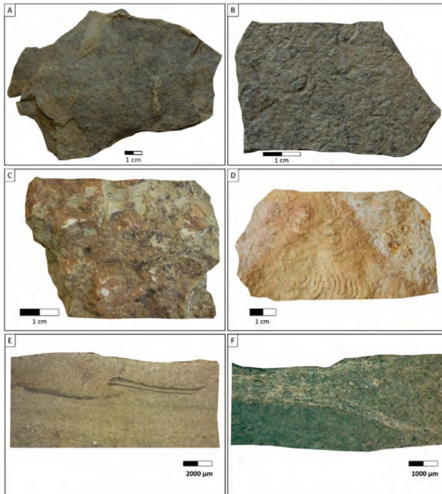
Fig. 3. Vendian deposits from sedimentary Formations of Volyno-Podillya basin showing MISS structures on their surfaces: A, B, C - siltstones from FN Formation (48°53', 27°48'); D - sandy silts from FM Formation (48°40', 28°00'); E, F - vertical section of silty sandstones from FM Formation (48°59', 27°46') whose contain clayey microbial micro-layer.
