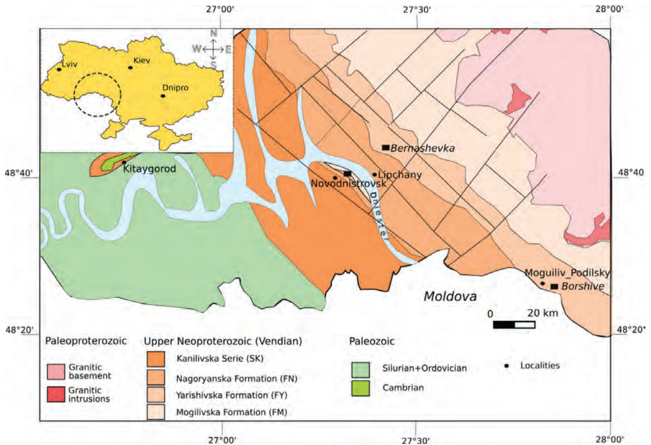
Fig. 1. Synthetic geological map showing the Paleozoic-Precambrian sedimentary cover and the Ukrainian Crystalline Shield.
