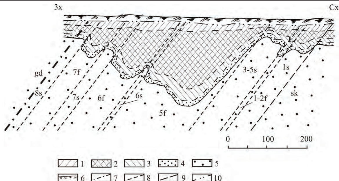
Fig. 3. Schematic geological section of the weathering rind of productive and containing layers of the Hannivsk deposits.
