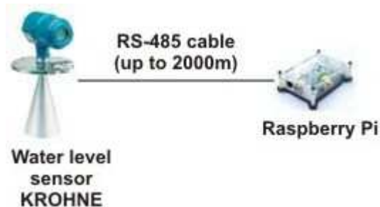
Figure 4 – Wiring of the water level sensor KROHNE to the Raspberry Pi computer
