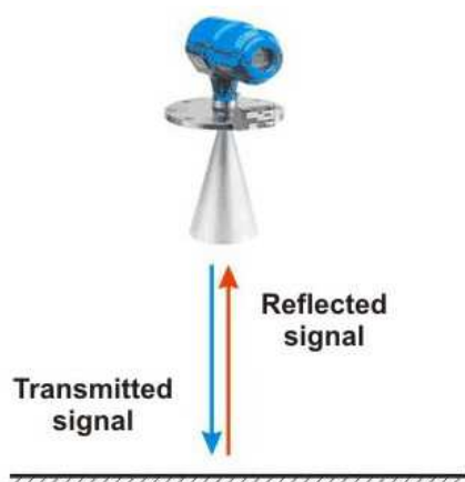
Figure 2 – Level Sensor KROHNE BM 70 A
