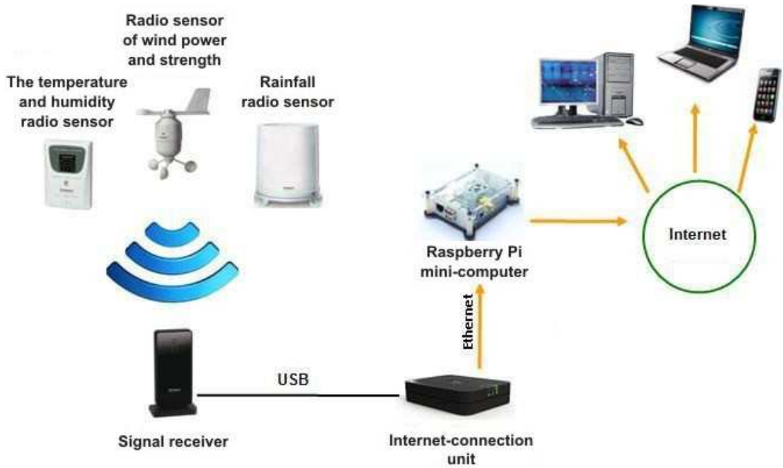
Figure 5 – Connection of components of the weather station OREGON LW301
