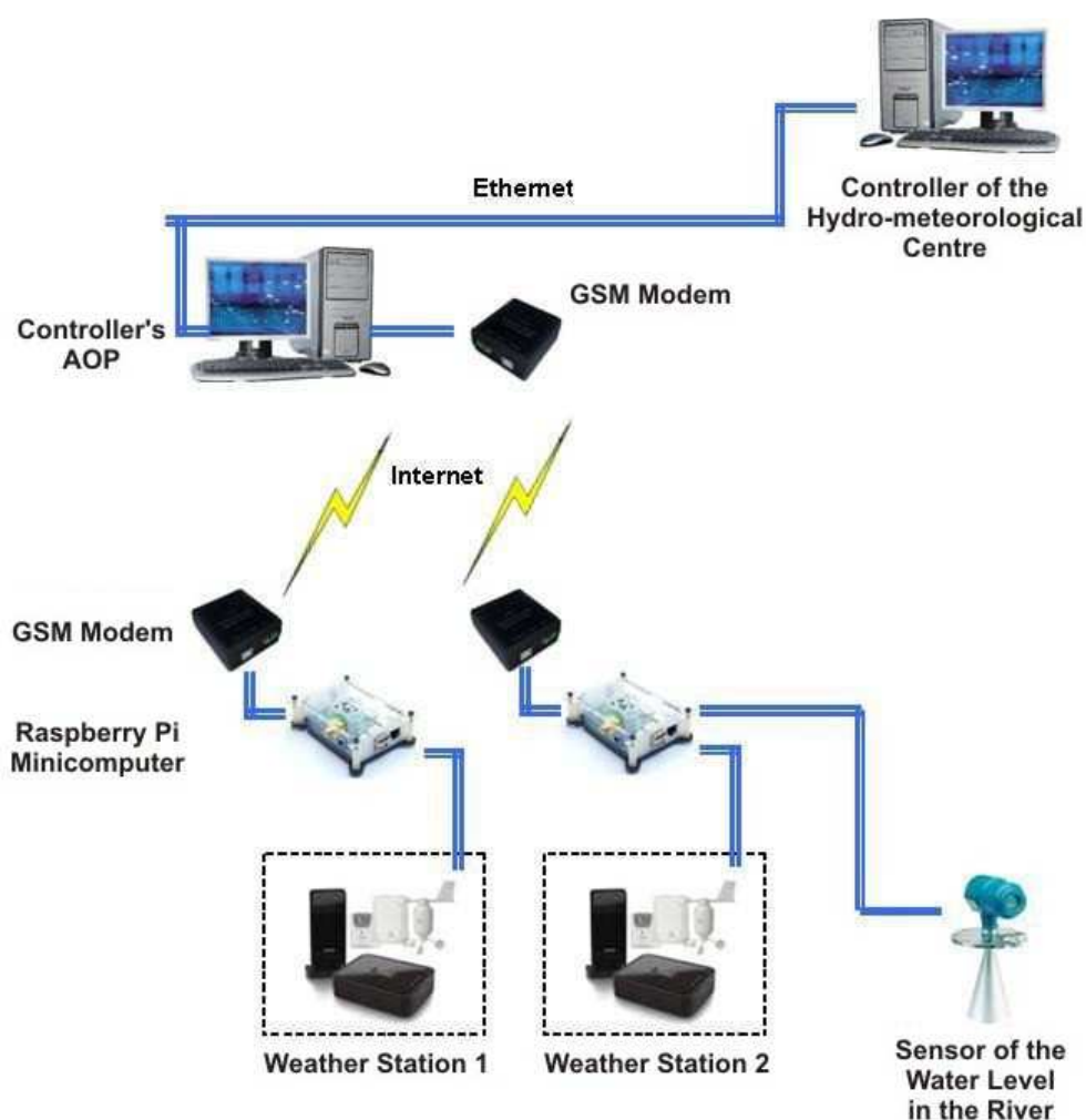
Figure 1 – Block diagram of a computer system
