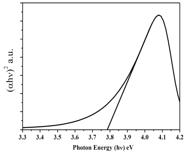
Fig. 6 – The plot of (\alpha h\nu)^2 vs h\nu for SnO 2 nanocrystallites
