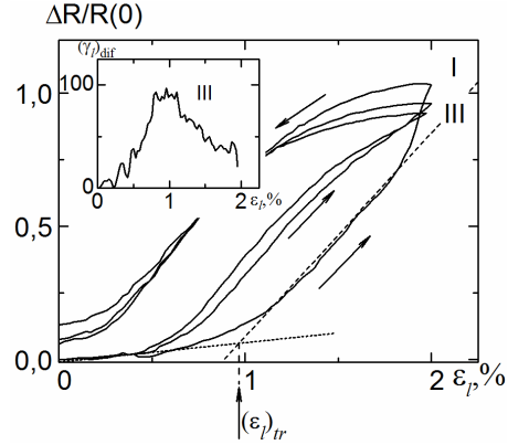
Fig. 7 – To explain the methodology the determination of \epsilon_{tr} based on strain dependency. On the insert- dependence (\gamma)_{dif} versus \epsilon_l for s.s.Au(Fe) at the concentration c_{Fe} = 70 at.%. I – III – the numbers of strain cycles
