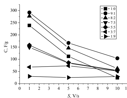
Fig. 2 – Specific capacity as function of voltage scan rate for pure \beta -Ni(OH) 2 and \beta -Ni(OH) 2 /C composites with the composition relationship \beta -Ni(OH) 2 :C = 90:10, 80:20, 70:30, 50:50, 30:70, and 10:90
