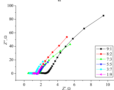
Fig. 7 – Nyquist diagrams for pure \beta -Ni(OH) 2 (a) and composites with different carbon content (b)
