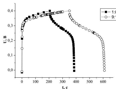
Fig. 4 – Charge-discharge curves of the pure \beta -Ni(OH) 2 and \beta -Ni(OH) 2 /C nanocomposite with the composition relationship 90:10
