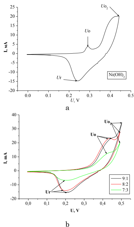
Fig. 3 – CVA of pure \beta -Ni(OH) 2 (a) and composites (b) at a voltage scan rate of 1 mV/s
