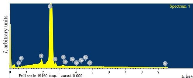
Fig. 3 – The electronic spectrum of Bi (0.150 at. % Te)
