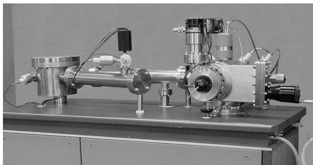
Fig. 1 – View of the time-of-flight mass spectrometer
