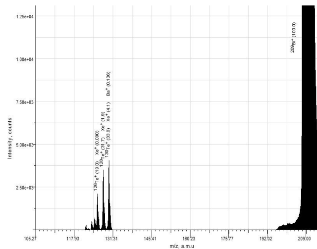
Fig. 2 – Mass spectrum of Bi (0.150 at. % Te). Combined cathode. The material of cathode wall is Al. Pressure 1.6 Torr. Gas mixture composition: Ar – 69.70 %, He – 30 %, H 2 – 0.30 %
