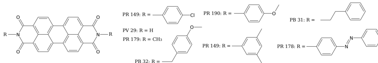
Fig. 1 – Chemical structure of PDI dyes
