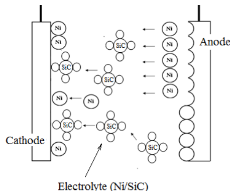
Fig. 2 – Co-deposition process
