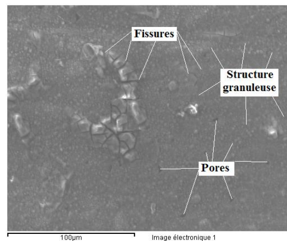
Fig. 7 – Surface morphology of N/SiC composite deposit in the presence of 25 g/l of SiC
