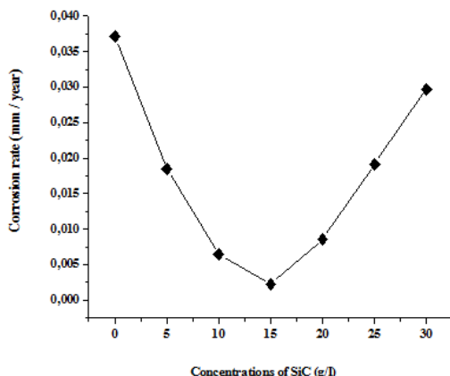
Fig. 3 – Corrosion rate of the specimens as a function of different SiC concentrations
