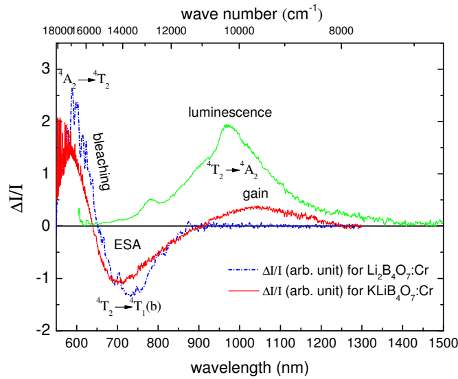
Рис. 1. Luminescence and ESA/gain/bleaching spectra of the \text{Li}_2\text{B}_4\text{O}_7:\text{Cr} and \text{KLiB}_4\text{O}_7:\text{Cr} glasses.
