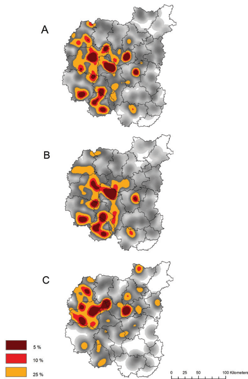
Figure 4. Rabies hotspots derived from kernel density estimation at three different thresholds (upper 5, 10, and 25% of density values), Chernihiv Oblast, 2011–2016: A — total cases, B — cases in domestic animals, C — cases in wild animals
