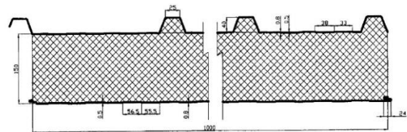
Fig. 2. The geometrical dimensions of the roof panel of the “AluTerm” series (cross-section) submitted for testing.
