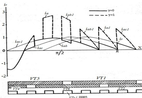
Figure 3. The oscillogram of a phase current of rotor of AEM in case of impulse control
