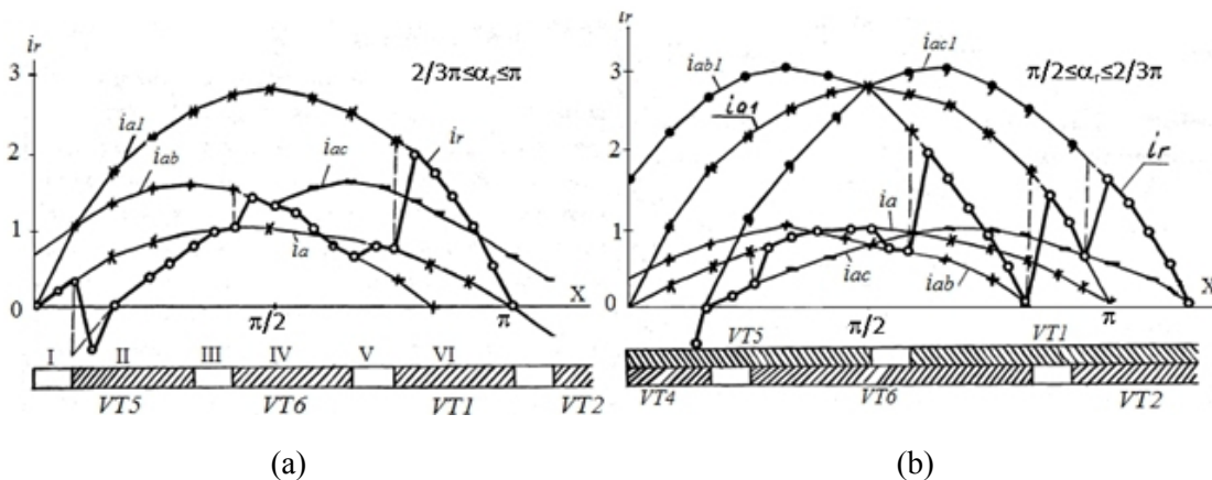
Figure 1. The oscillogram of a phase current of rotor of AEM in case of parametric control (a - the mode 0-1, b - the mode 1-2)
