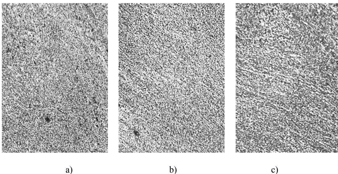
Figure 2. Microstructure of 01UT after HPT N=5, d=15 mm; x250
