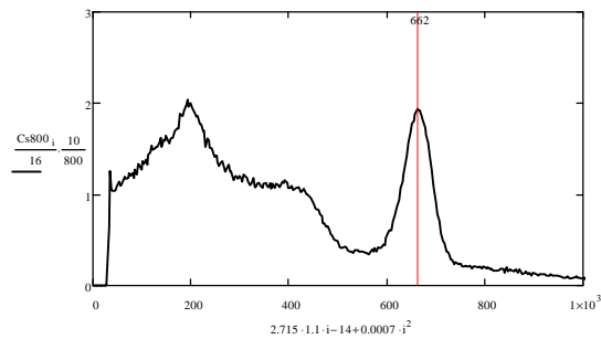
Figure 3. Hardware response spectrum for gamma detector CsI from 137 Cs at the UDD-Inter unit with several tungsten alloy attenuators
