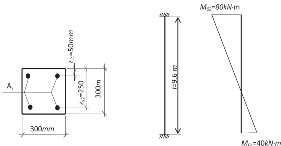
Fig. 5 Geometric parameters of column for calculation
