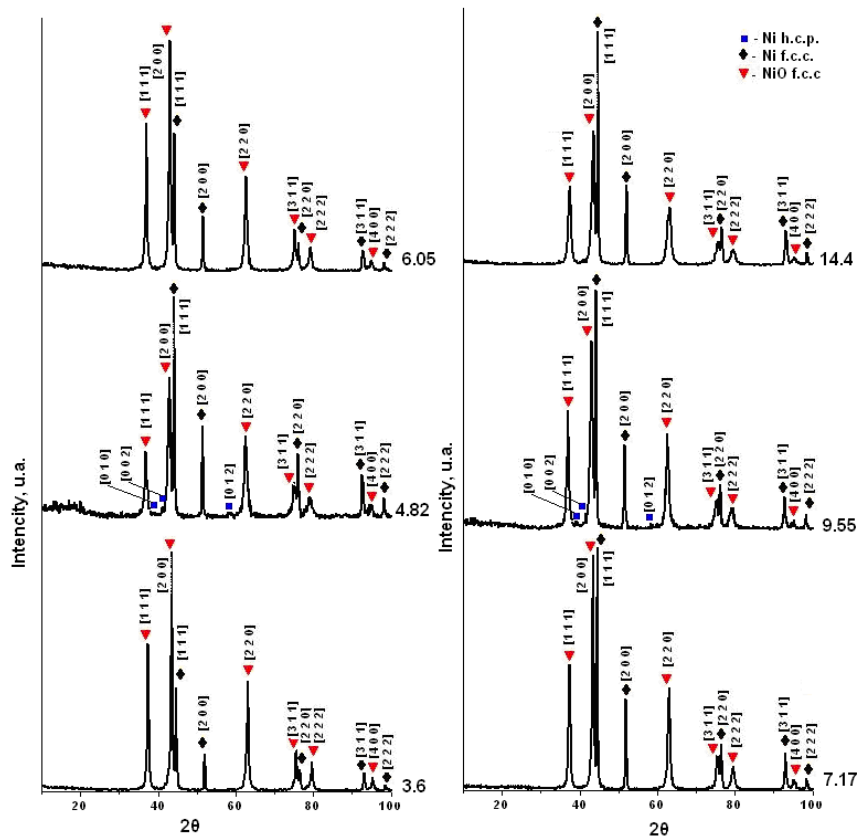
Fig. 3 – XRD patterns of Ni/NiO nanopowder obtained at different ammonia content in initial complex
