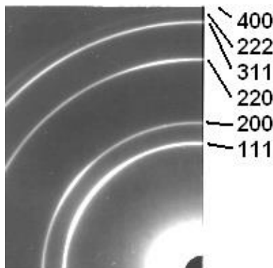
Fig. 1 – Electron diffraction pattern of film Ni
