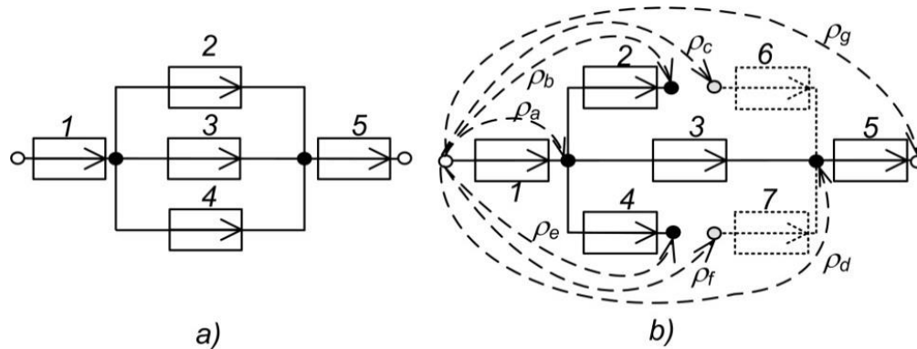
Fig. 1. The model of the IMS network
