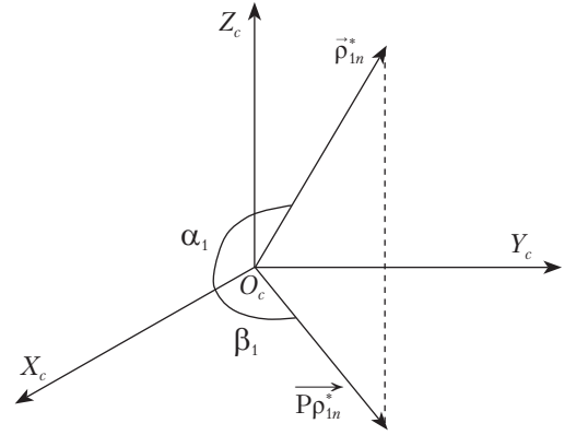
Fig. 3. Orientation of radius vector \vec{p}_{1n}^* in CCS
