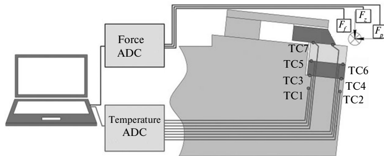
Fig. 1. Schematic view of the experimental setup.
