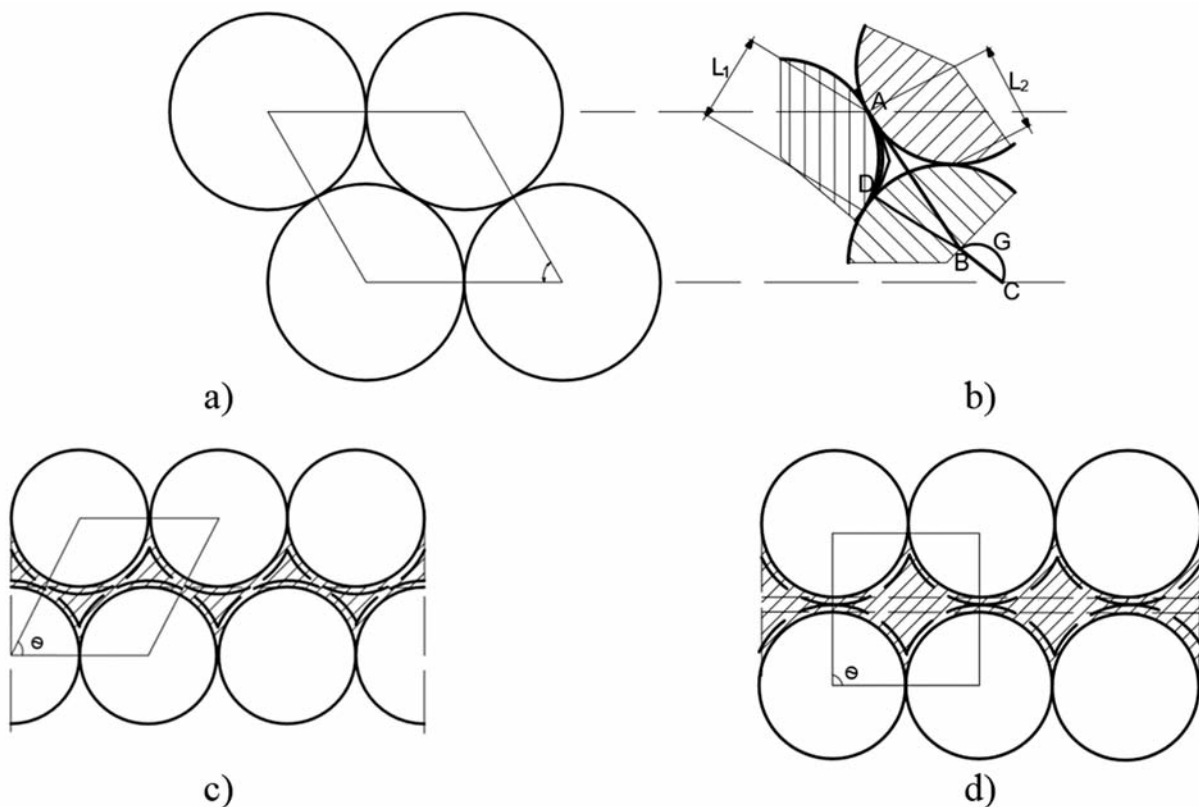
Figure 2. Location of the mineral particles in the fictitious ground:
