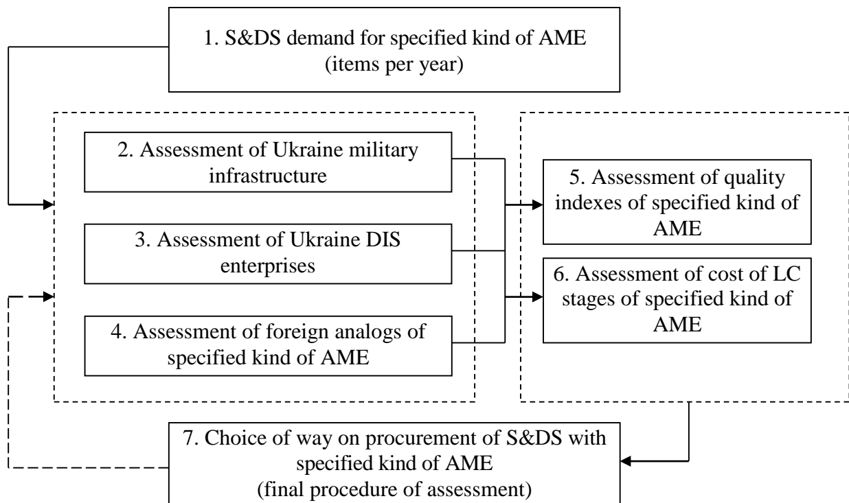
Fig. 1. Algorithm for analysis of factors (criterion) influencing on choice of way on procurement with specified AME in accordance with determined demand
