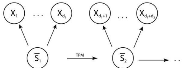
Fig. 4. Basic Structure of HSMM
