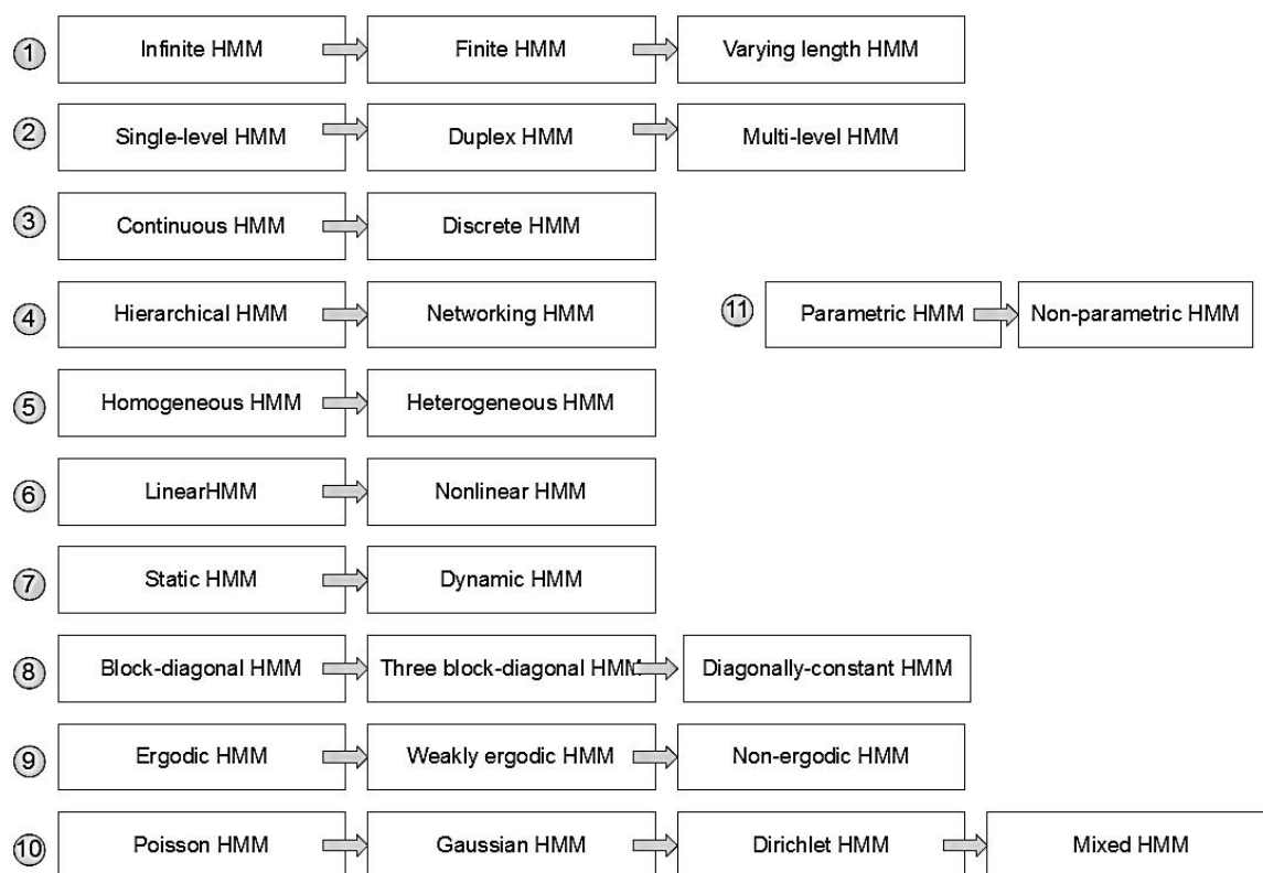
Fig. 5. The general scheme of classification of classical hidden Markov models.
