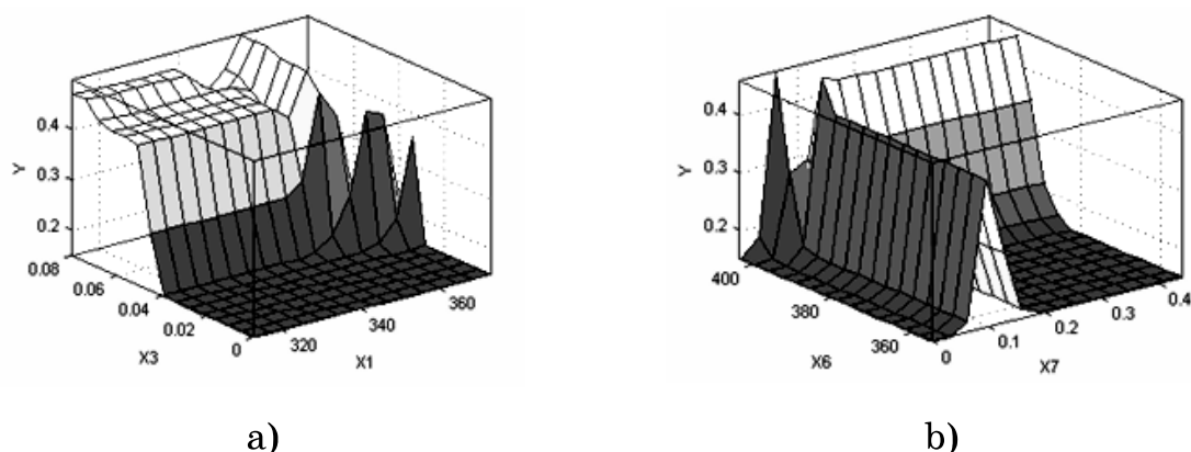
Fig. 1 - Dependence of the technical condition of the engine on the values of the input parameters: a) x_3 – «prelubricating pressure», x_1 – «air temperature after air cooler»; b) x_6 – «temperature after cylinders (high temperature cooling water system)», x_7 – «pressure before engine (low temperature cooling water system)»
