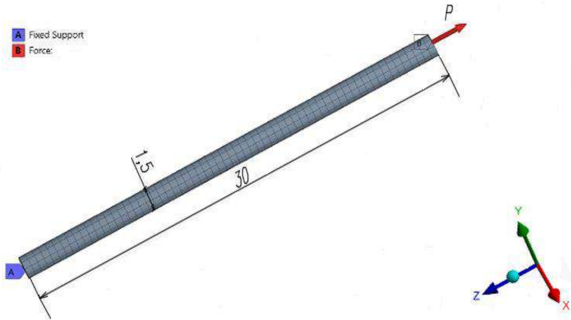
Figure 3. The finite element 3D model of wire
