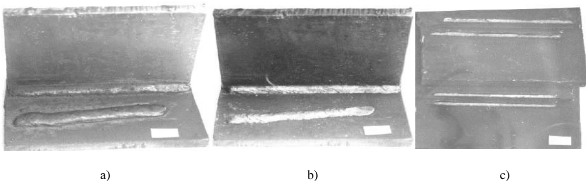
Figure 6. Bead appearance and a fillet weld (a) weld bead smallscaly formation (b) kinks fillet welds (c) formed researched ( d_e = 5,0 \text{ mm} ) electrodes type ET-2 with exothermic mixture in a coating
