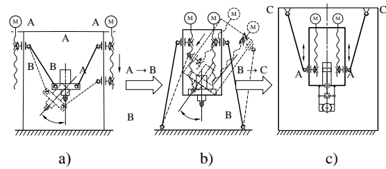
Fig. 1 – Circuit realization inversion for new properties manipulation systems with MPS (a) - traditional glide-layout; (b) – drives and carriage are moved to the mobile platform; (c) – rods fastening are transferred to another (any) surface [7]
