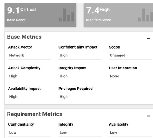
Figure 11 – An example of CVSS calculation
