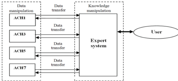
Figure3 – Logical structure of seven-tier LM-modefilter optimized with KB CAD system
