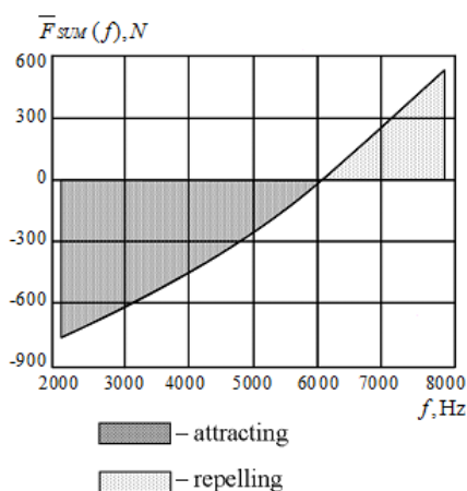
Fig. 2. An average integral force acting on the thin-walled ferromagnetic sheet as a function of the frequency of acting field
