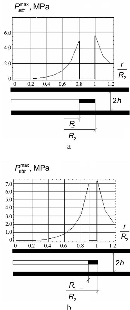
Fig. 6. The distribution of the density of attraction forces at the time moment when they have their maximum values for the following combinations of the dimensions of the inductor: a – R_1=0,035 m, R_2=1/0,8 \cdot R_1 ; b – R_1=0,035 m, R_2=1/0,9 \cdot R_1
