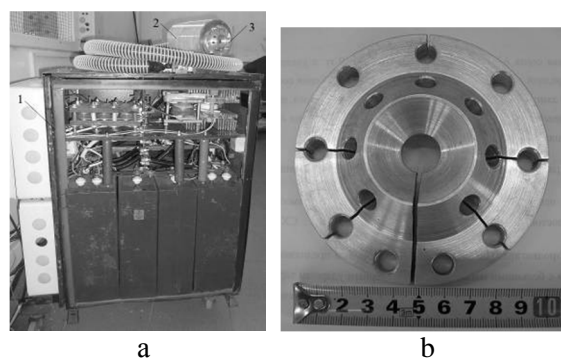
Fig. 3. The experimental setup: a – the laboratory equipment for EMF attraction processes with maximum charging voltage of 2kV and accumulated energy of 2kJ: 1 – pulse generator; 2 – pulsed current transformer; 3 – single turn inductor; b – the single turn massive inductor
