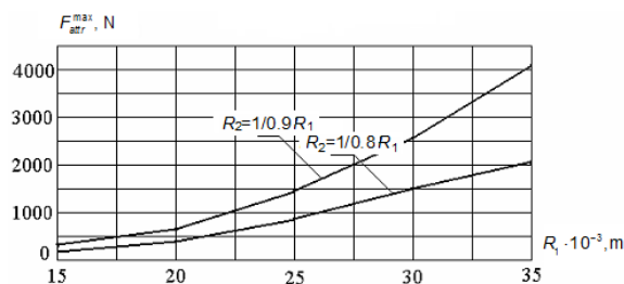
Fig. 7. The effect of the inner radius of the inductor on the attracting force between the screen and the blank
