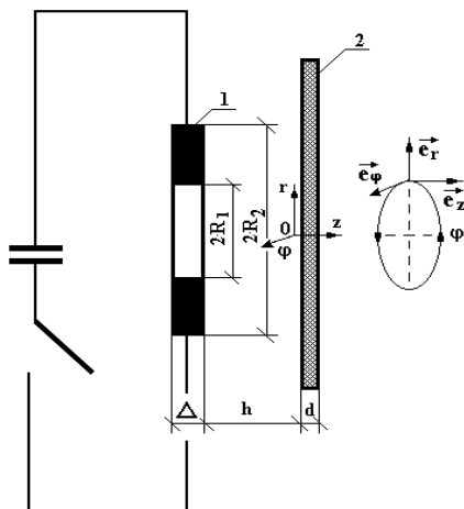
Fig. 1. The schematic of the single turn inductor (1) interacting with ferromagnetic sheet metal blank (2), where \vec{e}_r, \vec{e}_\phi, \vec{e}_z – are the unit vectors in the cylindrical coordinate system
