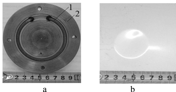
Fig. 8. The laboratory version of the ISAS (a, 1 – is the inductor, 2 – is the screen) and result of the EMF attraction of the part of the stainless steel sheet (b)
