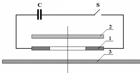
Fig. 5. Schematic of ISAS: 1 – is the single-turn inductor; 2 – is the auxiliary attracting screen; 3 – is the sheet metal blank; C – is the bank of capacitors; S – is the switch of the discharge circuit
