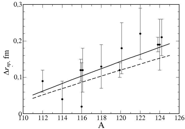
Fig. 5. Difference \Delta r_{np} between the rms radii of the neutron and proton distributions as a function of A for Sn isotopes. The solid and dashed lines are calculations with \eta=4 and 2 for SkM force. The experimental data are taken from Ref. [7].
