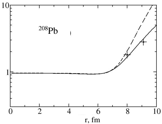
Fig. 6. The halo factor in ^{124}\text{Sn} and ^{208}\text{Pb} as a function of the distance from the center of the nucleus calculated using the Eq. (16). The values of the halo factor deduced from experiment are marked by crosses [7].
