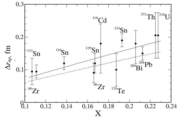
Fig. 4. Difference \Delta r_{np} between the rms radii of the neutron and proton distributions as a function of X = (N - Z) / A . The solid and dashed lines are calculations with \eta=4 and 2 for SkM parametrization of the Skyrme force. The experimental data are taken from Ref. [7].
