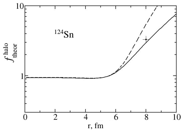
Fig. 6. The halo factor in ^{124}\text{Sn} and ^{208}\text{Pb} as a function of the distance from the center of the nucleus calculated using the Eq. (16). The values of the halo factor deduced from experiment are marked by crosses [7].
