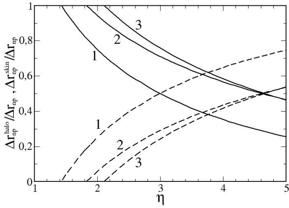
Fig. 3. The partial contribution to the isotopic shift of radii \Delta r_{np} from the skin effect, \Delta r_{np}^{skin}/\Delta r_{np} (solid lines) and the halo effect, \Delta r_{np}^{halo}/\Delta r_{np} (dashed lines) versus the parameter \eta . The calculations have been performed for ^{120}\text{Sn} with the following Skyrme force parametrizations: 1 - SIII; 2 - SkM; 3 - SLy230b.
