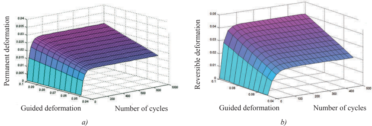
Fig. 2. Changing total deformations TSE during TSC: a — the residual strain; b — reversible deformation
